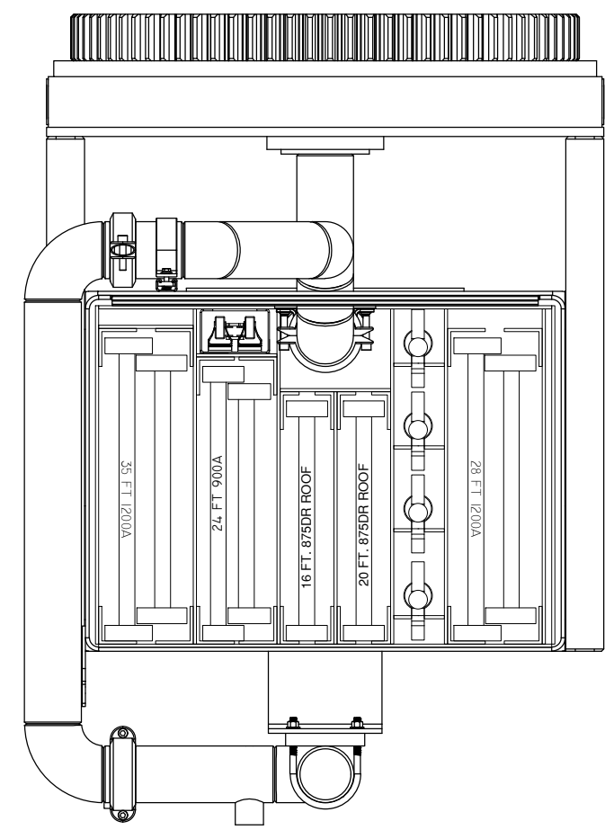
GROUND LADDER ARRANGEMENT
