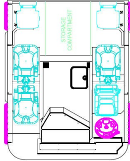
CAB INTERIOR PLAN VIEW
