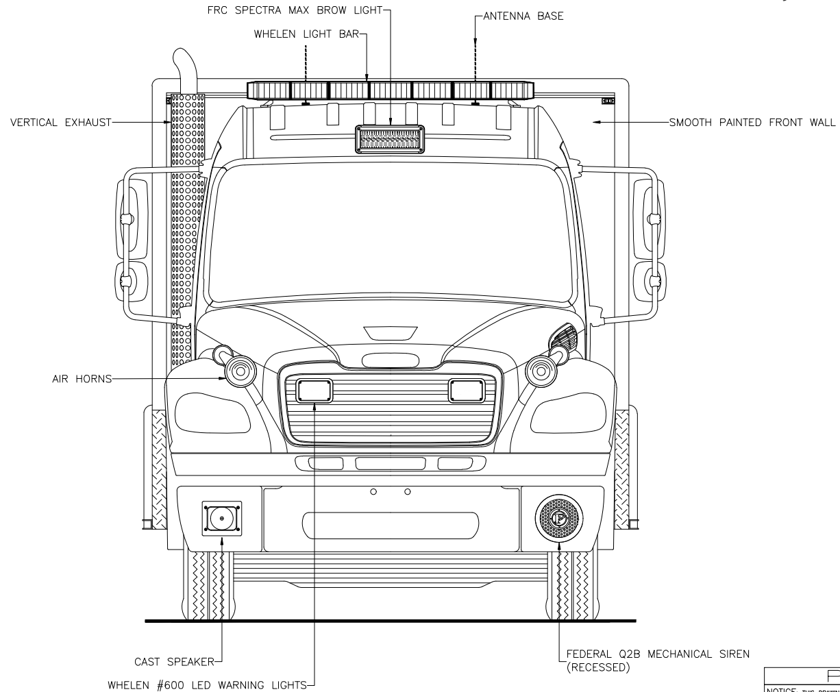
Front View
